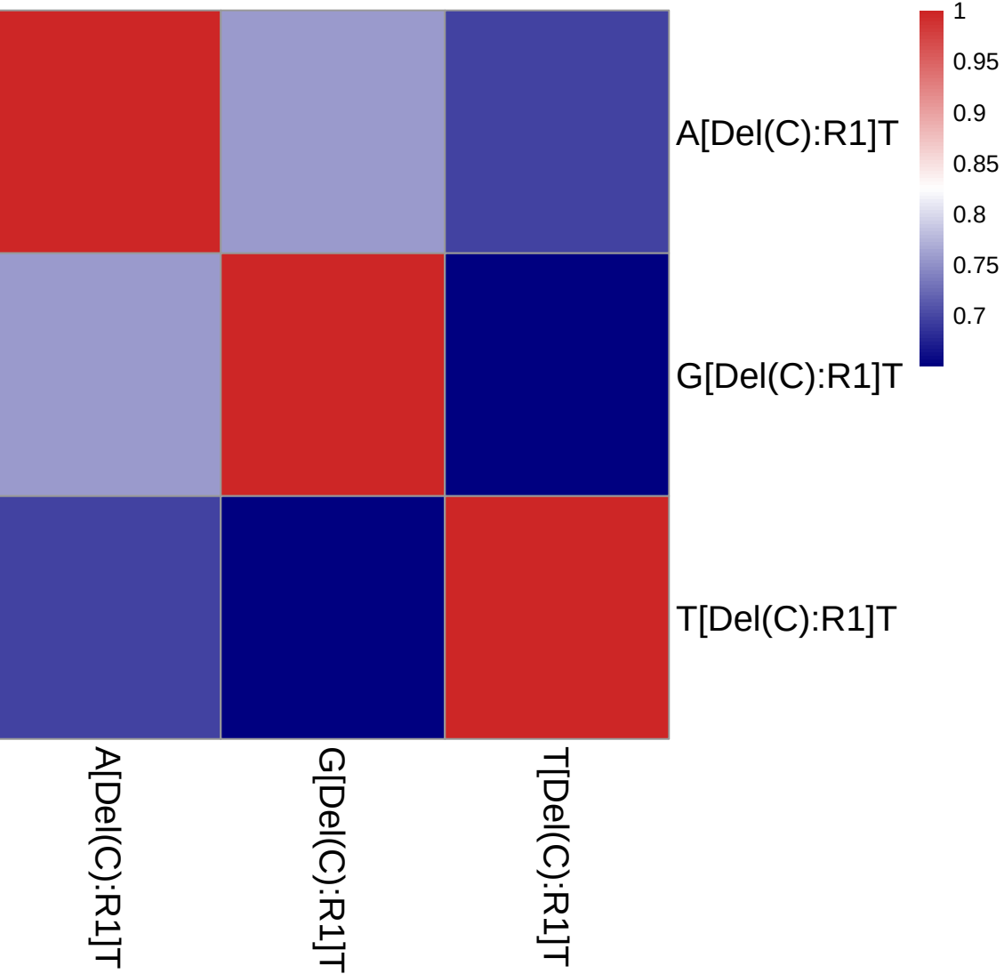
Heatmap – [Del(C):R1]T (Reordered by Base)
